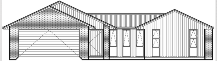
SOUTH EAST ELEVATION SCALE 1:100
