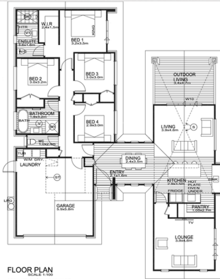
FLOOR PLAN SCALE 1:100
