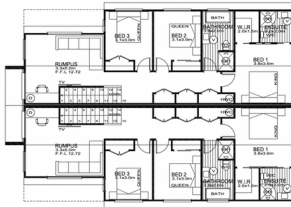
FLOOR PLAN L2 SCALE 1:100 AREA: 196.6m 2 OVER FRAMING
