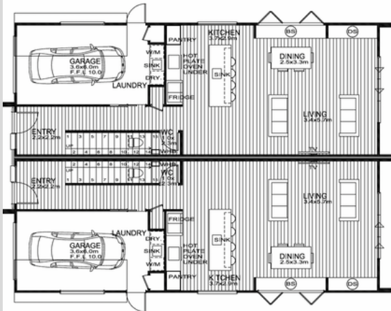
FLOOR PLAN L1 SCALE 1:100 AREA: 204.57m 2 OVER FRAMING
